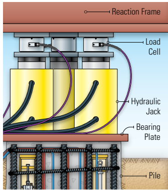
Load cells used in pile test.
