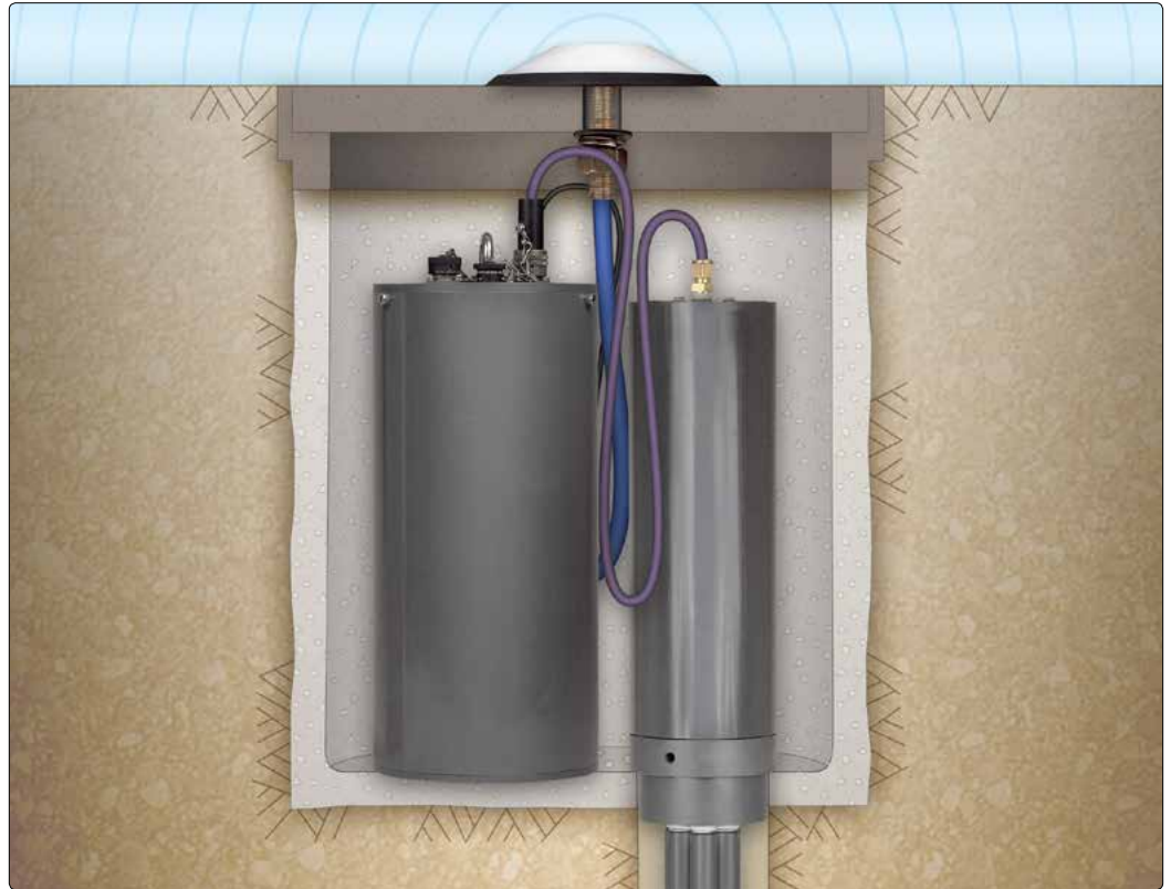
• Model 8026 Datalogger and Model 1150 (A-3) Extensometer in manhole, with manhole lid antenna.
