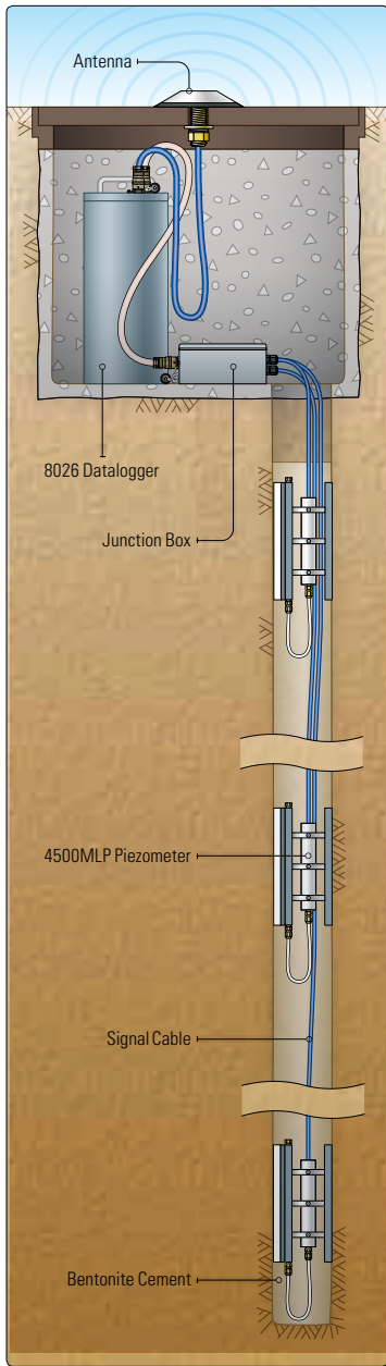
● Model 8026 Datalogger shown with Model 4500MLP Multilevel Piezometers.
