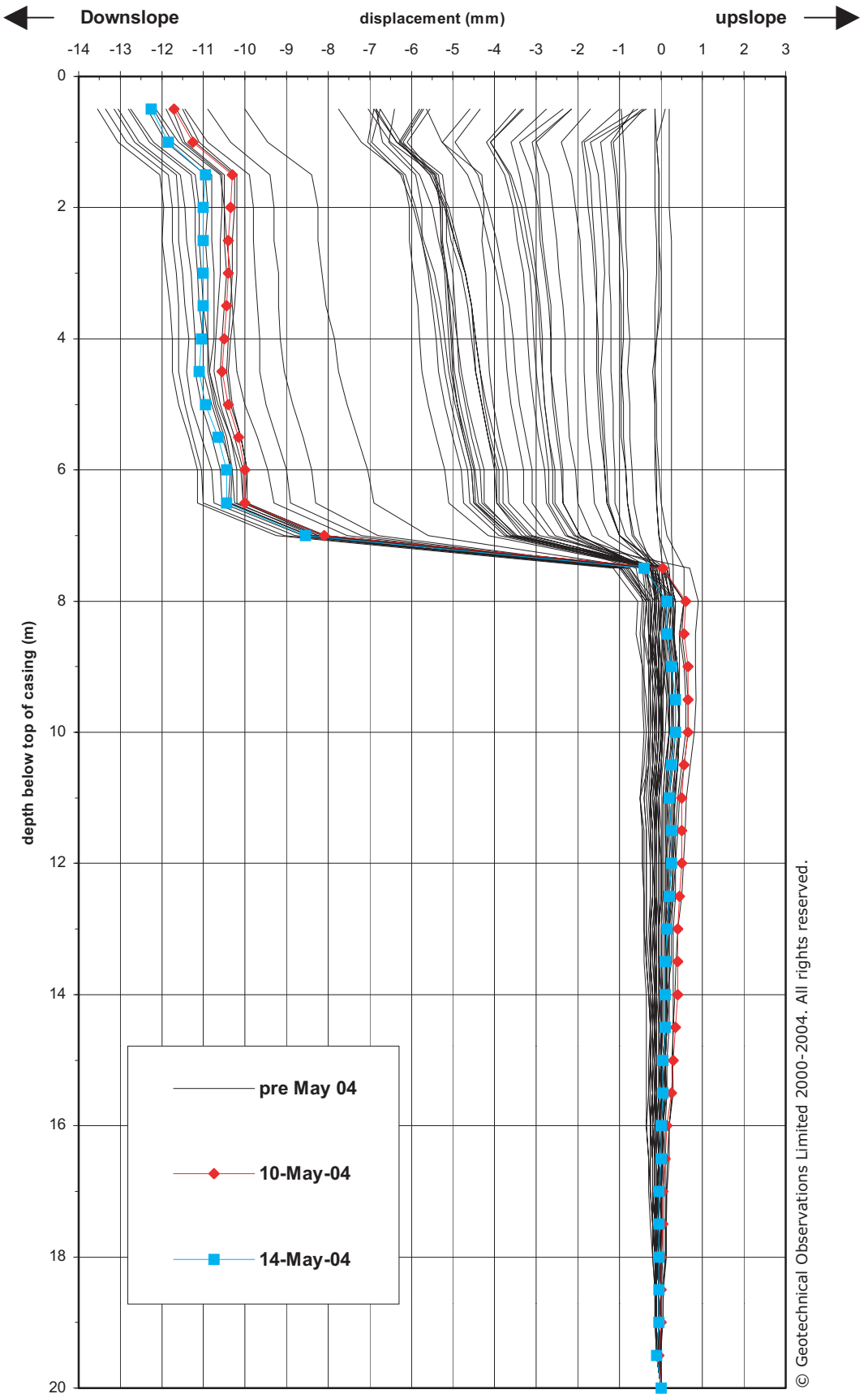
Figure 1: Manual Inclinometer Readings
