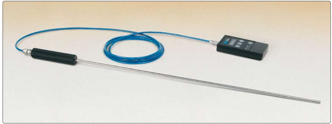
● Model 4910 Probe shown with the Geokon Model GK-404 Vibrating Wire Readout.
