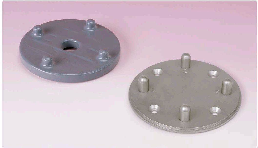
● Geokon Model 6201-1C Ceramic and 6201-1S Stainless Steel Tiltplates (tiltplates are permanently attached to structure being monitored).
