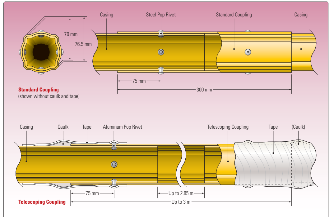
• Illustration depicts the Model 6500 Inclinerometer Casing dimensions, and configurations of the standard and telescoping couplings.
