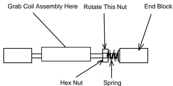
Figure 2 - Tension Adjustment
