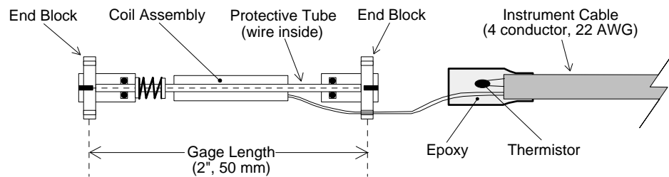
Figure 2 - Model 4202 Vibrating Wire Strain Gage
