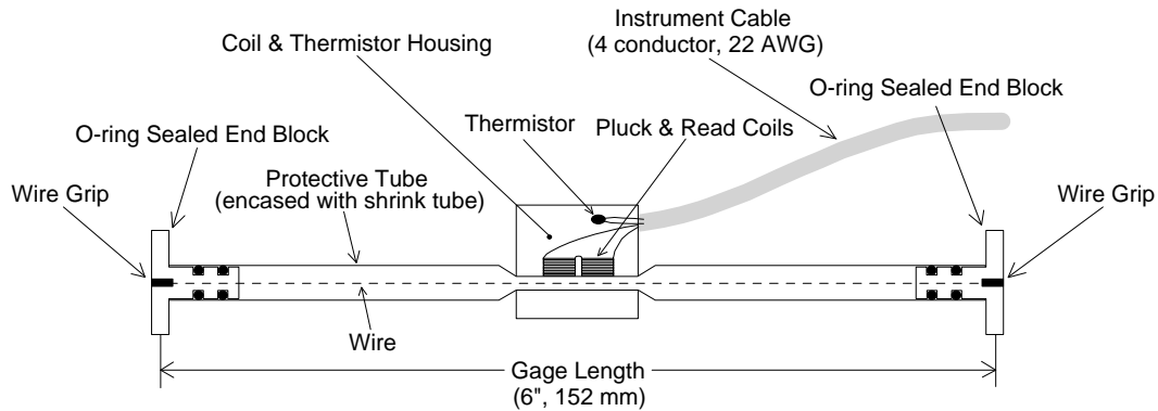
Figure 1 - Model 4200 Vibrating Wire Strain Gage
