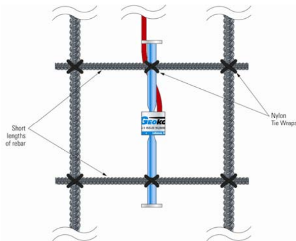
Figure 4B - Alternative Method for attaching Model 4200/4200HT straingages to rebar.
