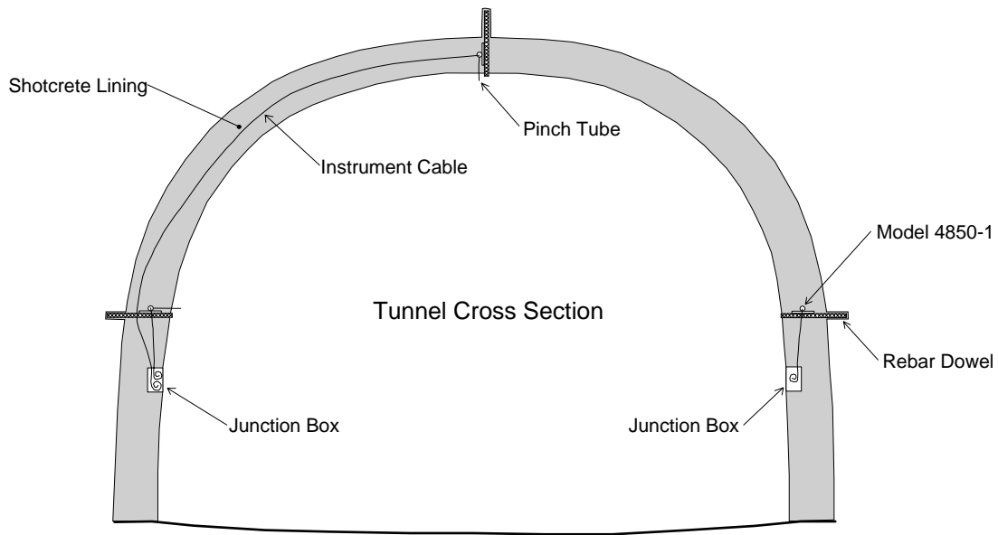
Figure 3 - Model 4850-1 Installation
