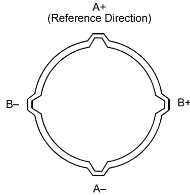
Figure 2. Inclinometer Casing
