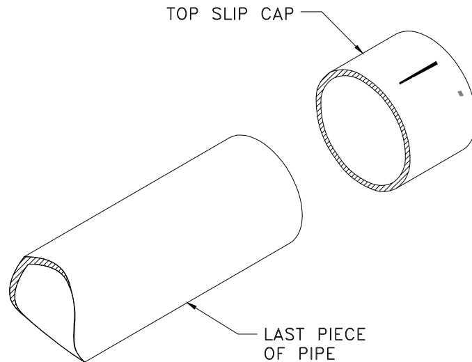
Figure 4 – Top Cap
