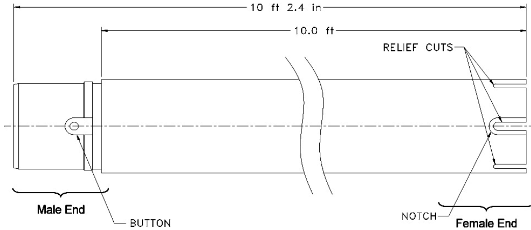
Figure 1 – Geokon Glue and Snap casing
