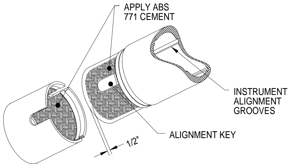
Figure 2 – End Cap Joint
