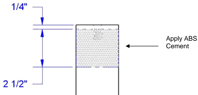
Figure 7 – Casing Preparation
