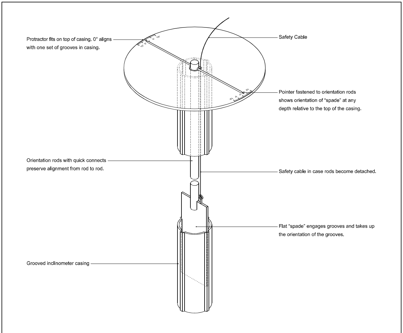
Figure 2. Model 6010 Spiral Sensor
