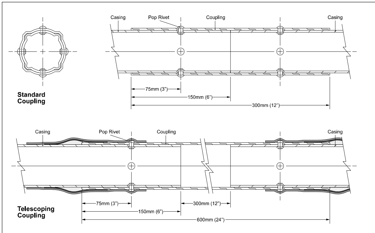
Figure 1. Inclinometer casing and couplings.
