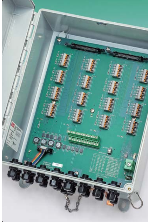
● Model 8032 Multiplexer (MUX).
