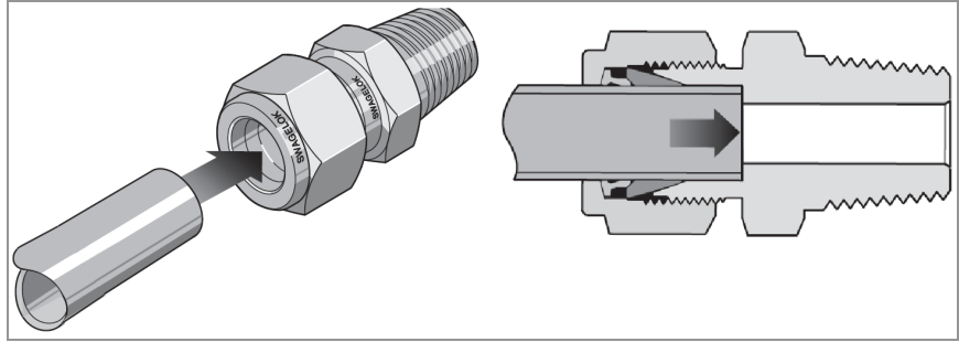
FIGURE 8: Tube Insertion
