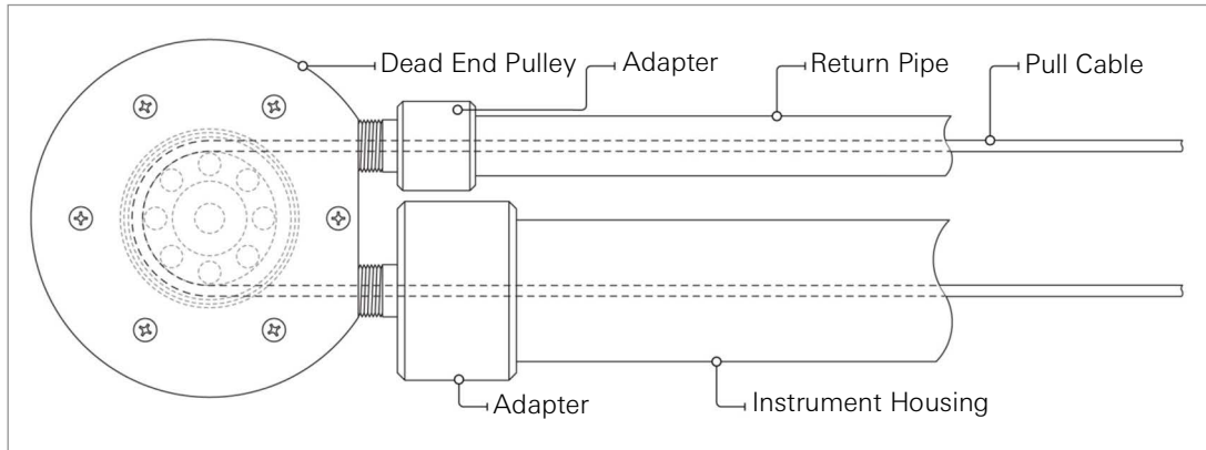
FIGURE 3: Dead End Pulley Diagram
