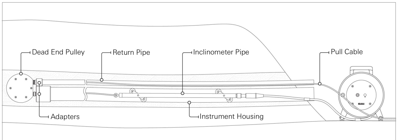
FIGURE 2: Horizontal Probe Using the Dead End Pulley System
