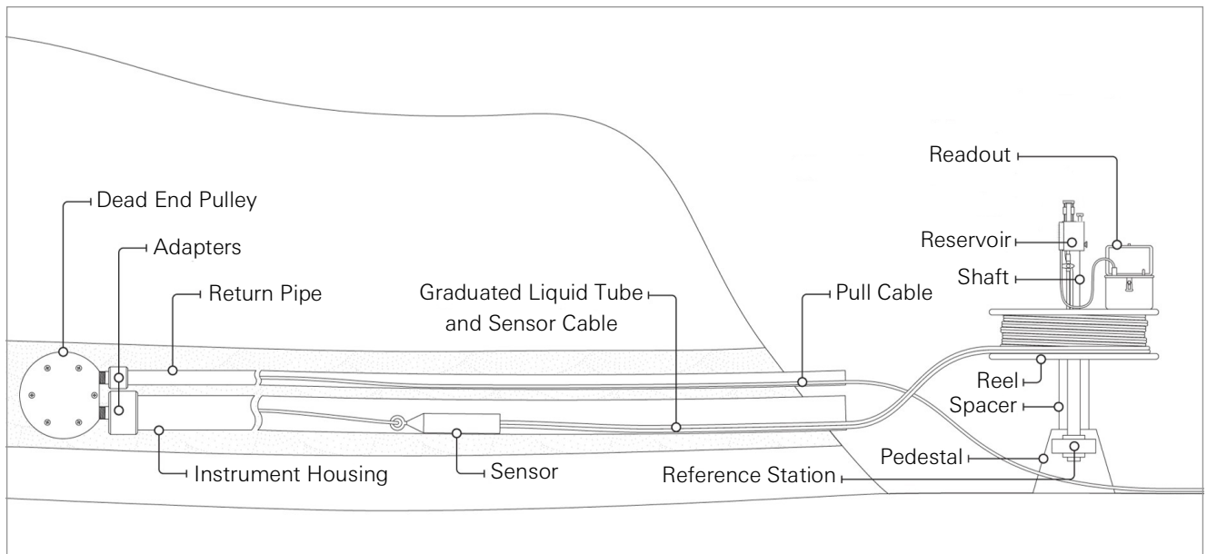
FIGURE 1: Settlement Profiler Using the Dead End Pulley System
