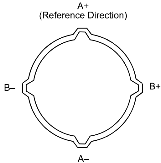
Figure 3 - Inclinometer Casing
