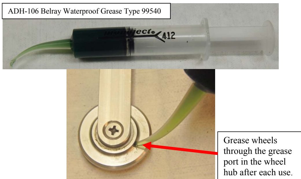
Figure 4 - Wheel Lubrication
