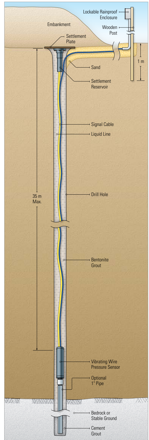
Typical Model 4600 installation.
